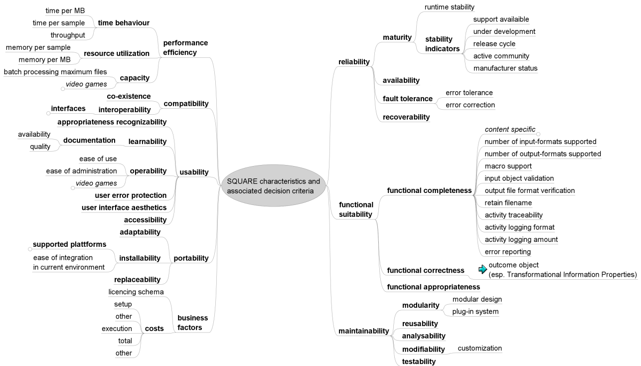
Figure 3: Metrics for SQUARE quality attributes
