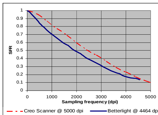
Figure 2. SFRs for scanners used in this study
